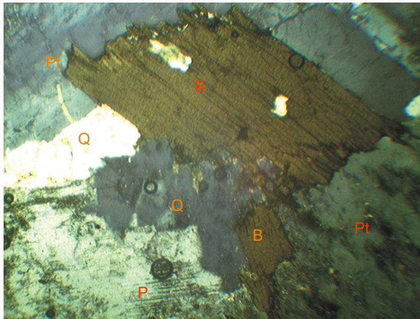
Figure 5. Photomicrograph of Syenite showing porphyroblasts of biotite (B) with inclusions of quartz (Q) surrounded by perthite (Pt) and plagioclase feldspars (P) (Cross polars x 4)
