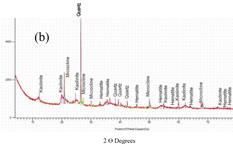
Figure 7. X-ray diffraction of (a) soil and (b) laterite developed on Syenite in Pankshin area
