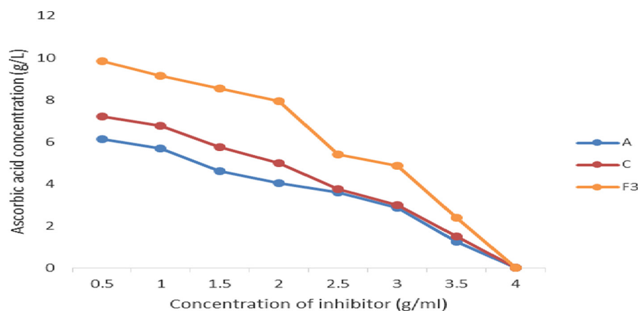
Fig. 7. Effect of inhibitor (EDTA) on ascorbic acid production by parent and fusant strain (F3) of Aspergillus flavus (A) and Aspergillus tamarii (C). F = 0.436 , P = 0.657 .
