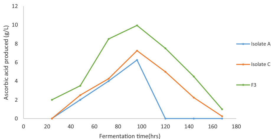
Fig. 3. Production of ascorbic acid by parent and fusant strain (F3) of Aspergillus flavus (A) and Aspergillus tamarii (C). F = 1.032 , P = 0.413 .
