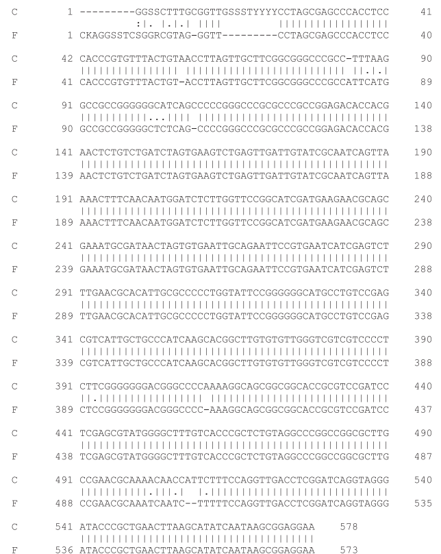
Fig. 2. Pairwise alignment of Aspergillus tamarii (C) and fusant (F) nucleotides.
