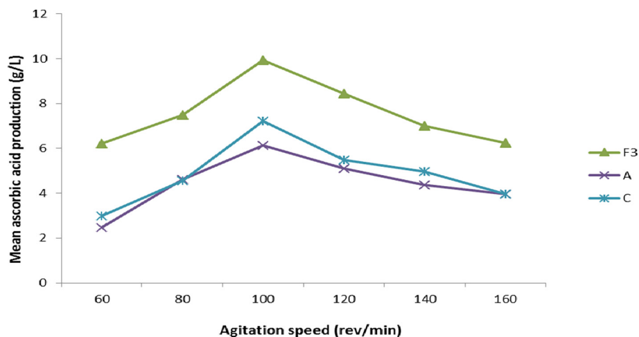
Fig. 6. Effect of agitation speed on ascorbic acid production by parent and fusant strain (F3) of Aspergillus flavus (A) and Aspergillus tamarii (C). F = 0.736 , P = 0.564 .
