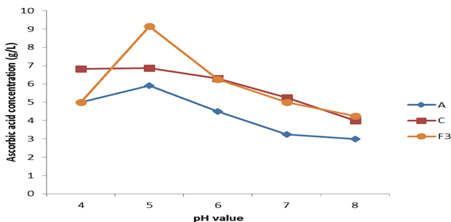
Fig. 4. Effect of pH on ascorbic acid production by parent and fusant strain (F3) of Aspergillus flavus (A) and Aspergillus tamarii (C). F = 1.812 , P = 0.205 .
