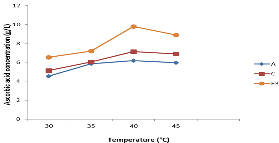
Fig. 5. Effect of temperature on ascorbic acid production by parent and fusant strain (F3) of Aspergillus flavus (A) and Aspergillus tamarii (C). F = 1.212 , P = 0.512 .
