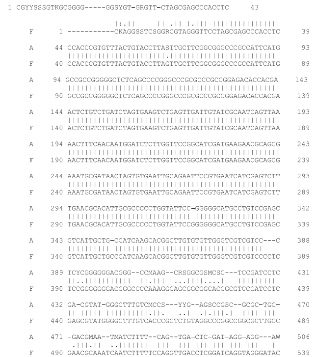
Fig. 1. Pairwise alignment of Aspergillus flavus (A) and fusant (F) nucleotides.
