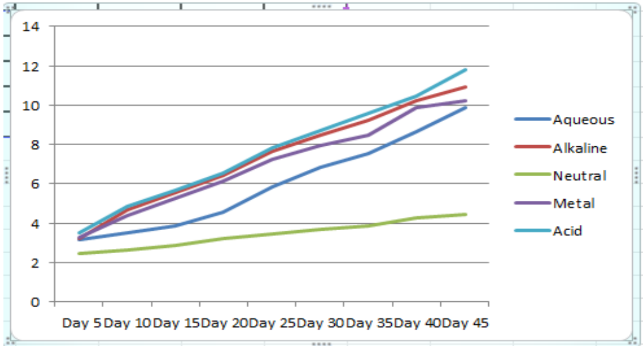
Figure 1: Plot of the Peroxide Value of the soybean oil sample over ten days in different environments
