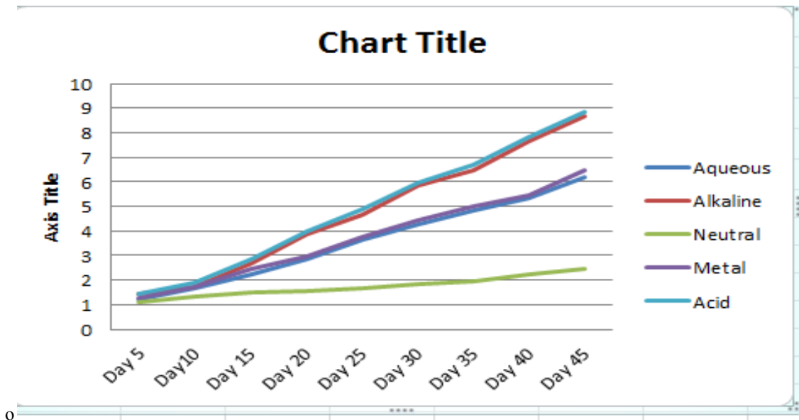
Figure 2: Plot of the % FFA of the soybean oil sample over ten days in different environments
