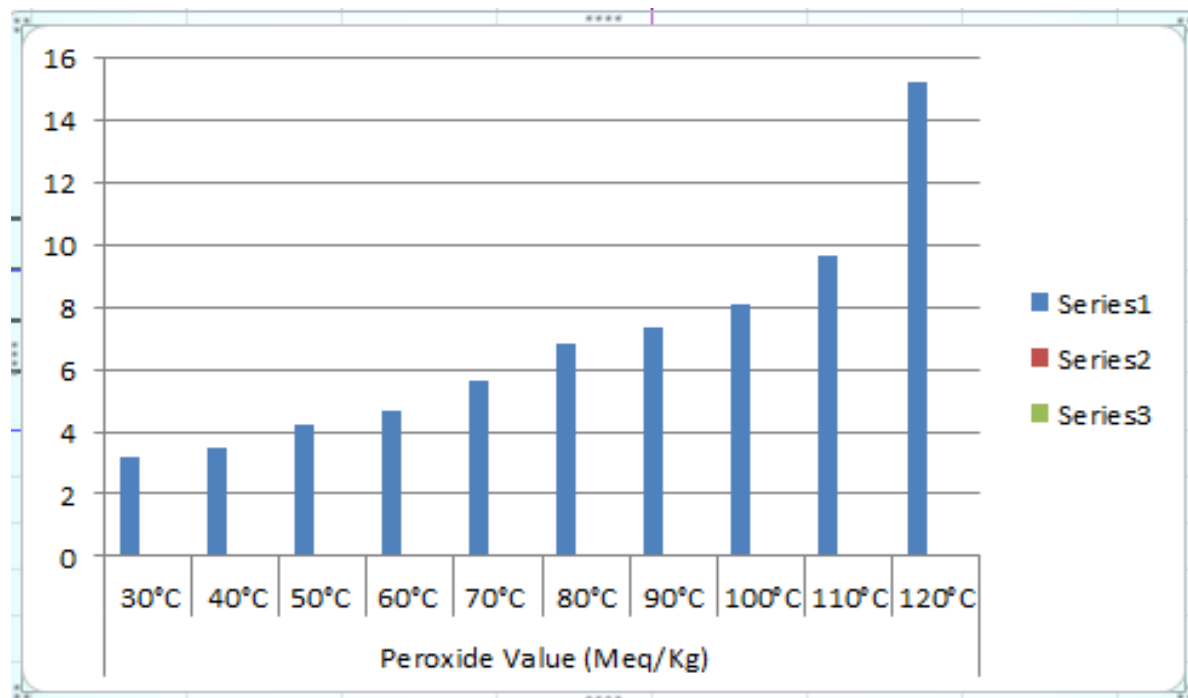
Figure 4. A histogram showing the effect of increasing temperature on the peroxide value of crude soybean oil.
