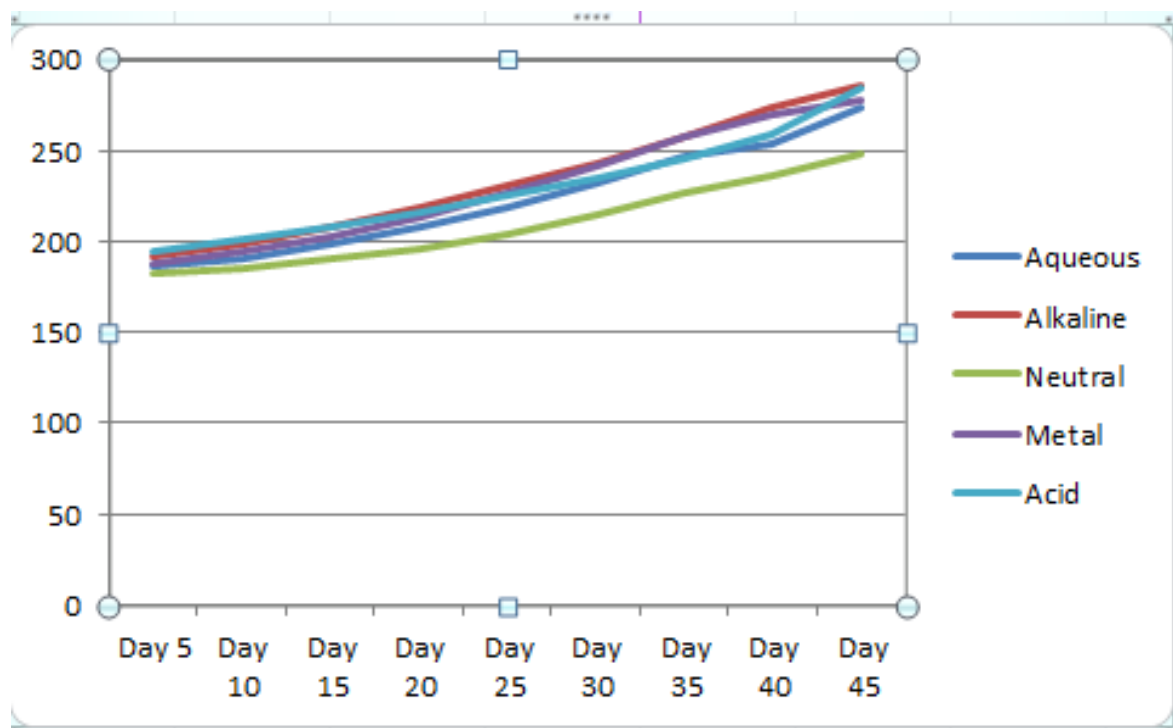
Figure 3: Plot of the Saponification Values of the soybean oil sample over ten days in different environments
