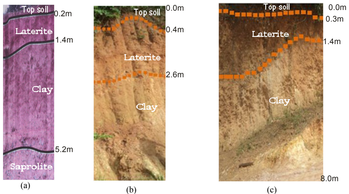
Figure 4. Weathered profiles of the study areas
