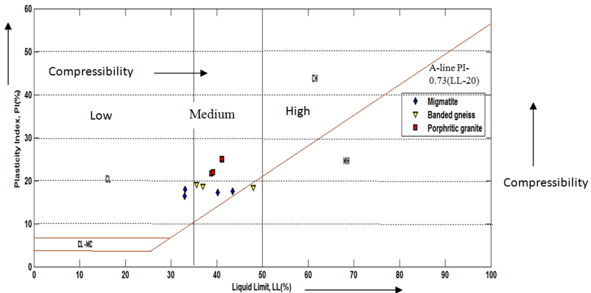
Figure 6. A plasticity chart for classification of the clay deposits (after Casagrande 1948)
