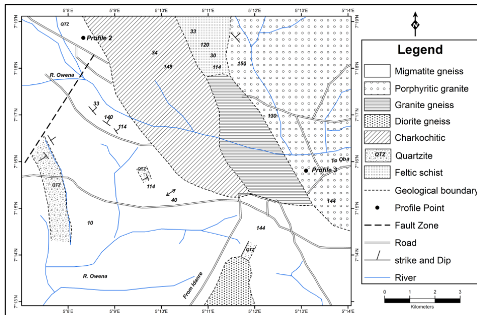
Figure 3. Geological map of Akure area showing clay sites
