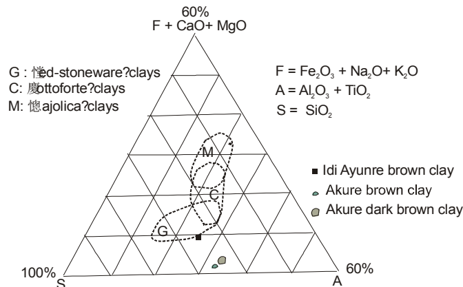
Figure 7. Ternary diagram SiO_2/Al_2O_3+TiO_2/Fe_2O_3 + MgO + CaO + K_2O + Na_2O ( After Fabbri and Fiori, 1985)
