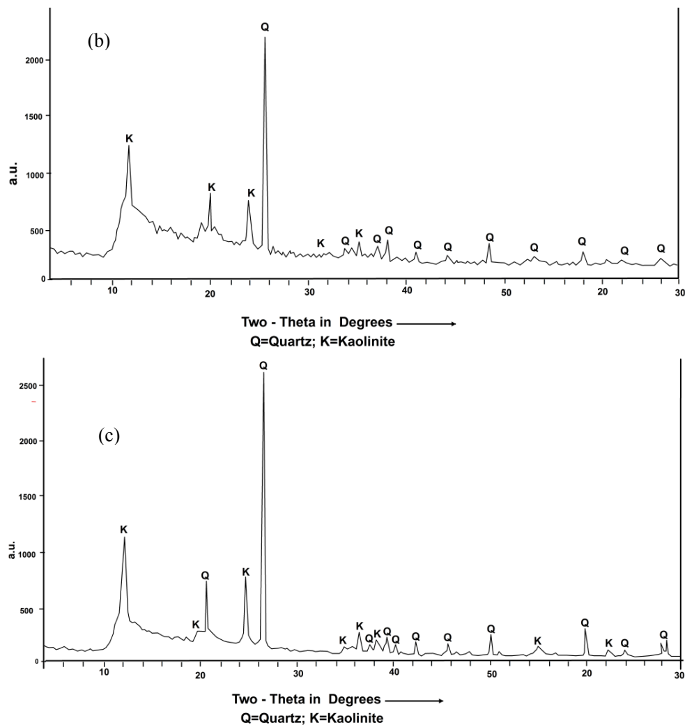
Figure 5. X-ray diffraction diagrams for the clays samples (a) -Idi-Ayunre brown variety, (b)-Akure brown clay, (c) - Akure dark brown body
